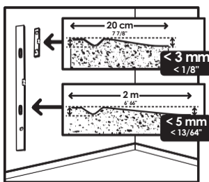
SUBSTRATE EVENNESS
